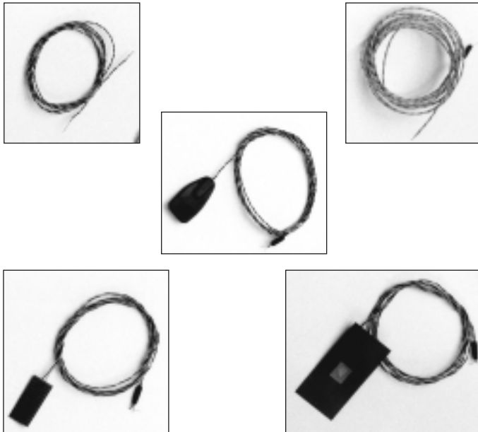
Fig 13: Thermocouples for Surface Temperature Sensing
